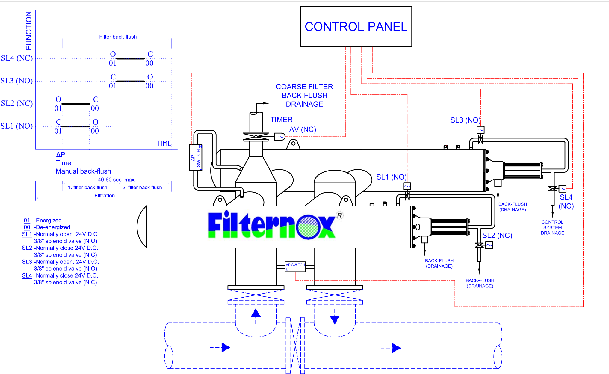
TYPICAL INSTALLATION AND ELECTRIC CONTROL SYSTEM CONNECTION DIAGRAM
